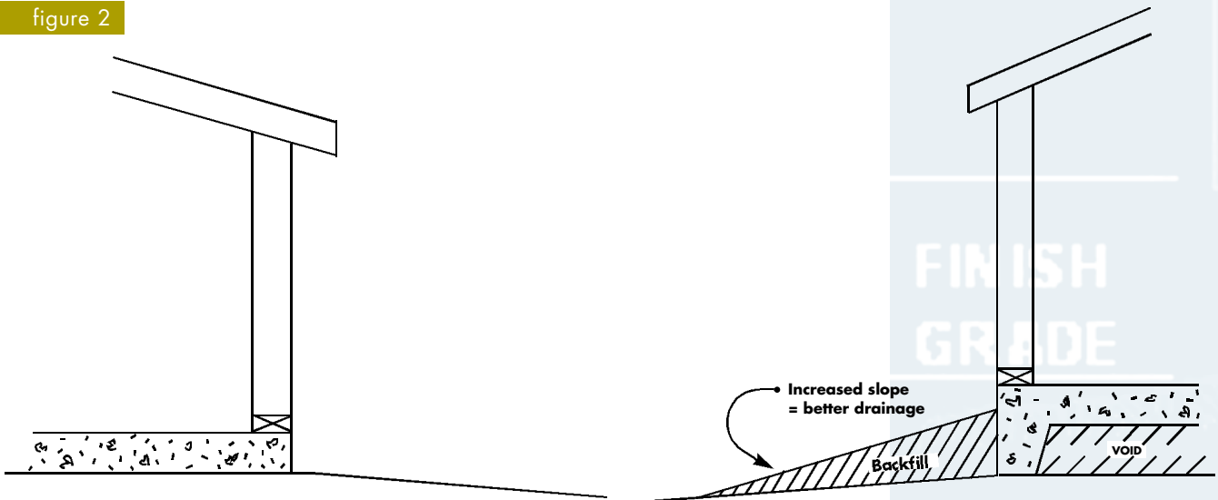
Figure 2: Backfill around taller WAFFLEMAT foundation increases slope, improves drainage.
